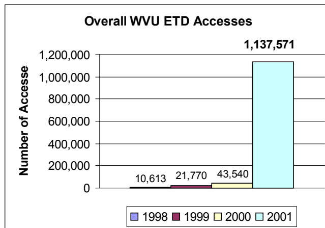
Figure 6 ETDs Accessed
