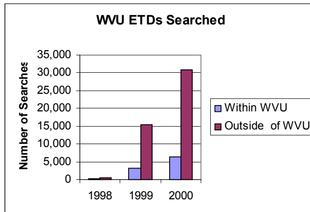
Figure 4 ETD Searches
